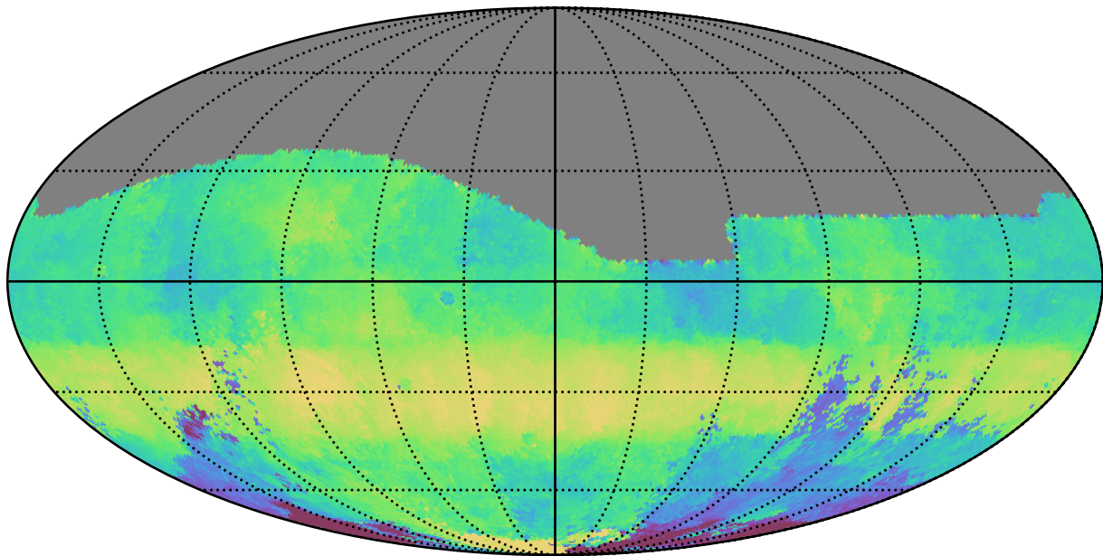
ddf_loaded_fl2_v3.4_10yrs All sky g band: Median HA
