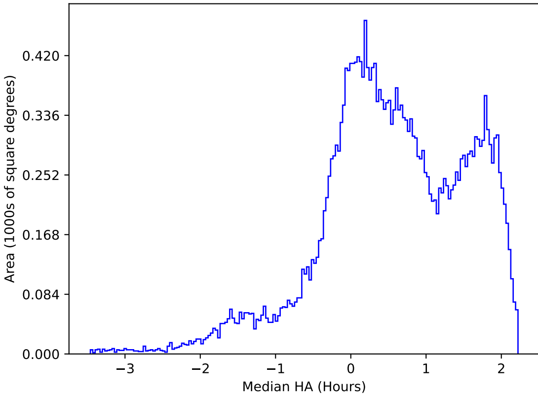
ddf_loaded_fl2_v3.4_10yrs All sky g band: Median HA
