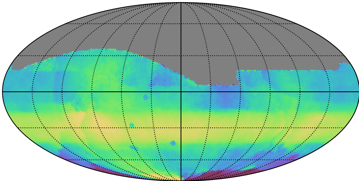
ddf_loaded_fl2_v3.4_10yrs All sky all bands: Median HA
