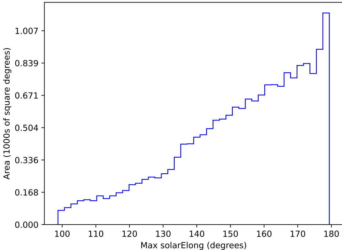
ddf_loaded_fl2_v3.4_10yrs WFD z band: Max solarElong
