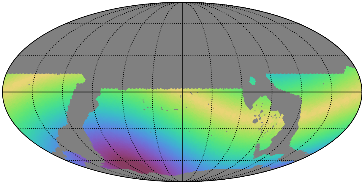
ddf_loaded_fl2_v3.4_10yrs WFD y band: Max solarElong
