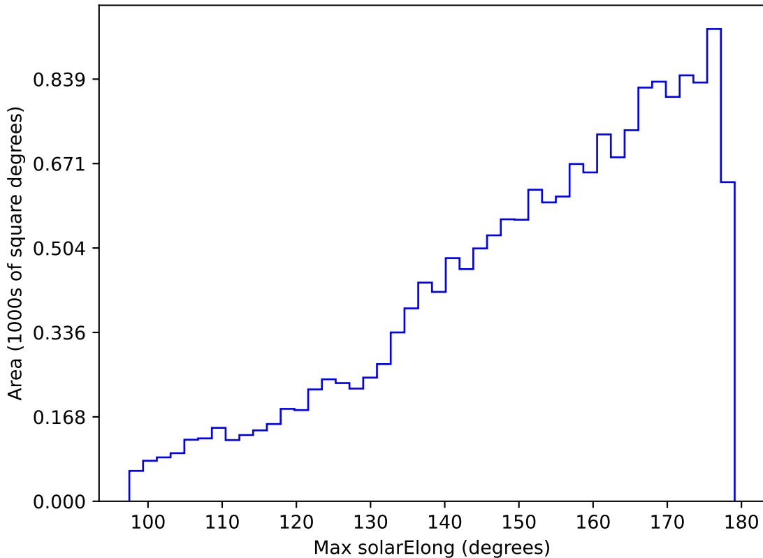
ddf_loaded_fl2_v3.4_10yrs WFD u band: Max solarElong
