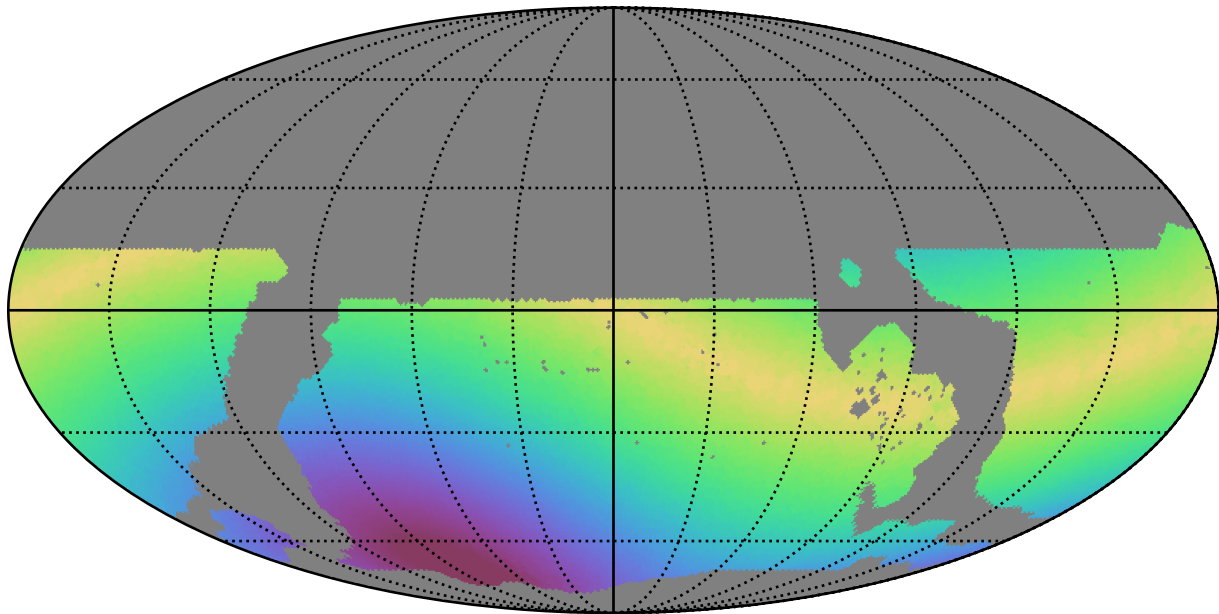
ddf_loaded_fl2_v3.4_10yrs WFD g band: Max solarElong
