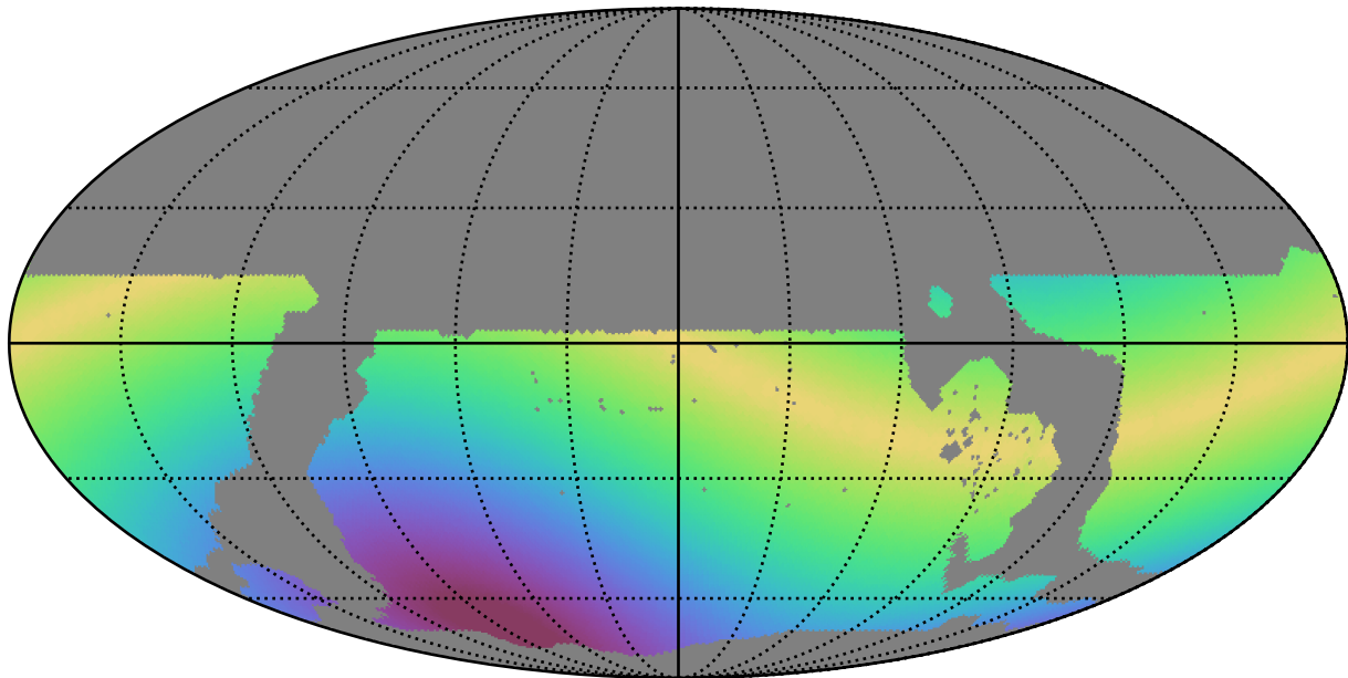
ddf_loaded_fl2_v3.4_10yrs WFD all bands: Max solarElong
