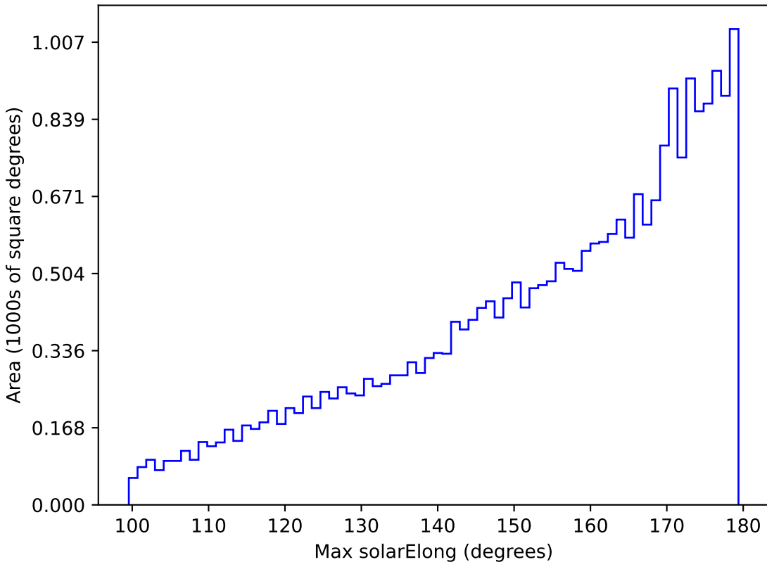
ddf_loaded_fl2_v3.4_10yrs All sky z band: Max solarElong
