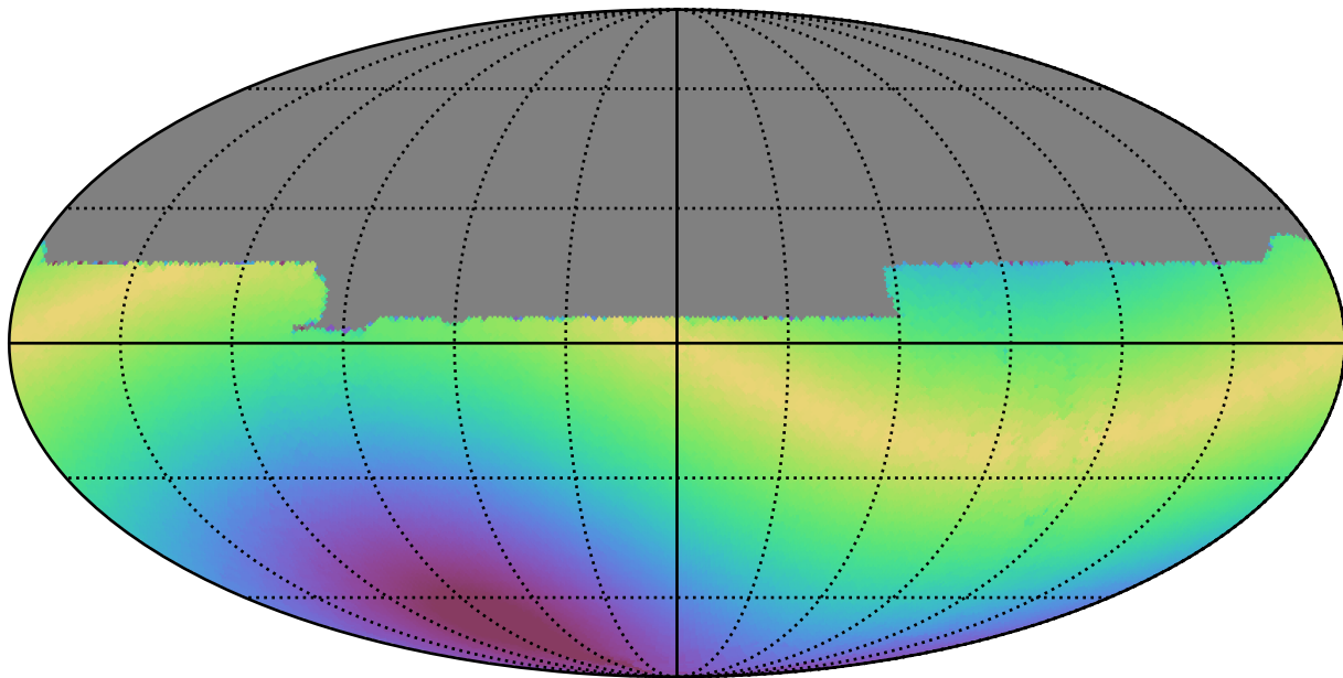
ddf_loaded_fl2_v3.4_10yrs All sky y band: Max solarElong
