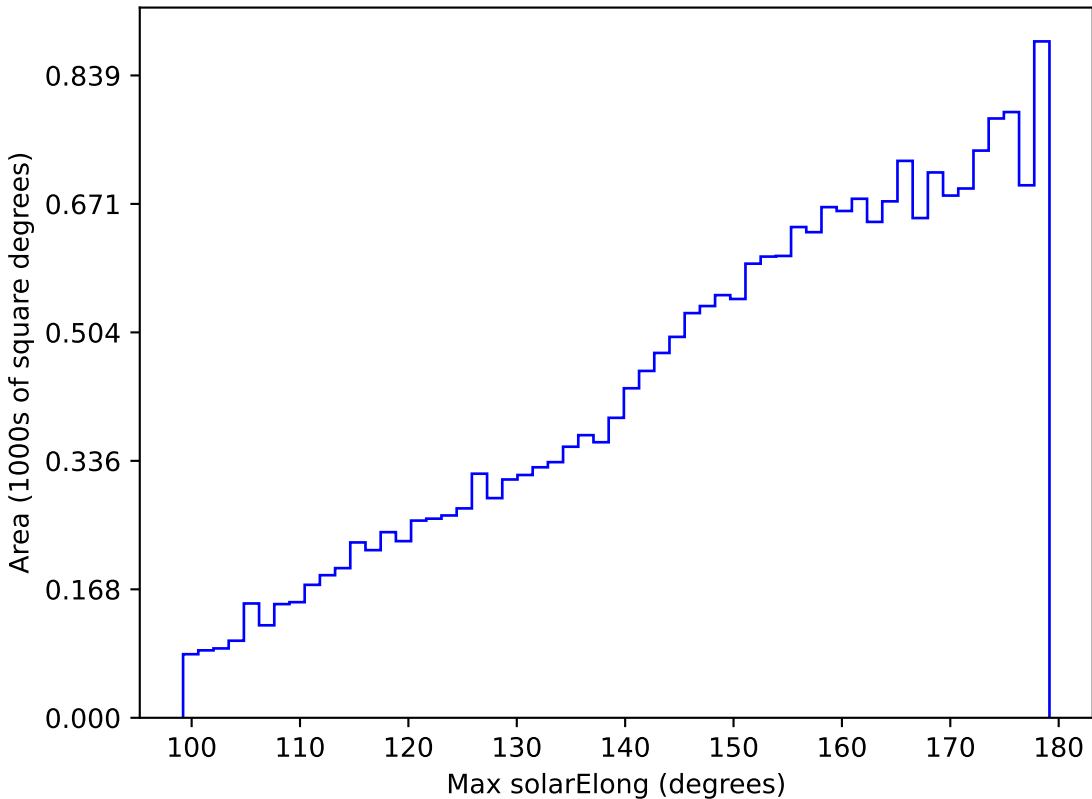
ddf_loaded_fl2_v3.4_10yrs All sky y band: Max solarElong
