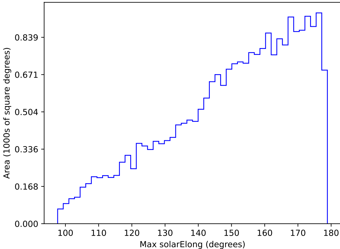
ddf_loaded_fl2_v3.4_10yrs All sky u band: Max solarElong
