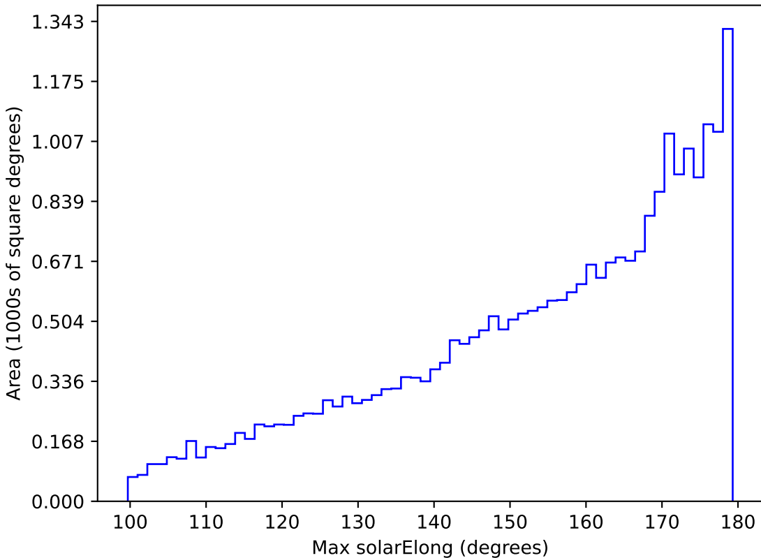
ddf_loaded_fl2_v3.4_10yrs All sky r band: Max solarElong
