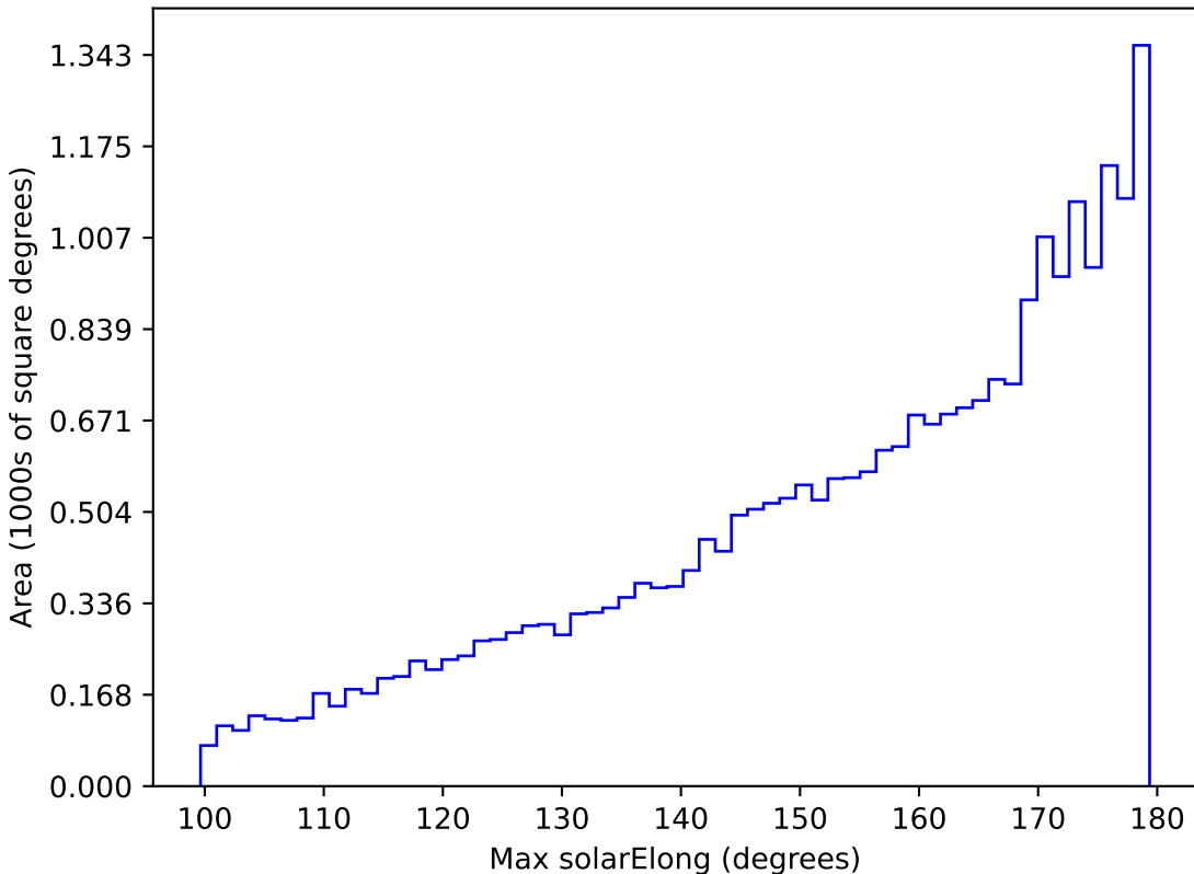
ddf_loaded_fl2_v3.4_10yrs All sky i band: Max solarElong
