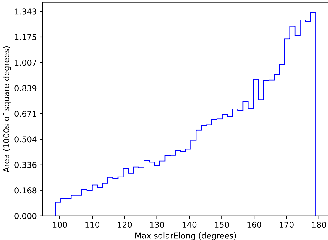
ddf_loaded_fl2_v3.4_10yrs All sky g band: Max solarElong
