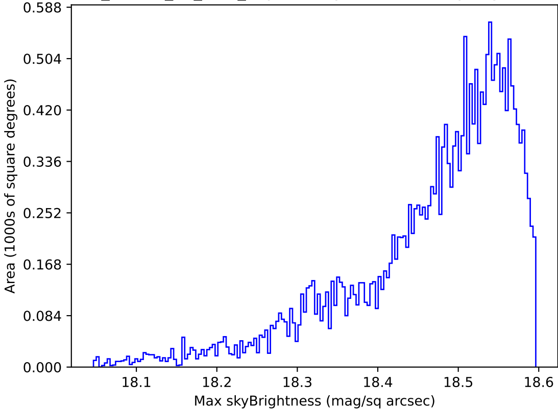
ddf_loaded_fl2_v3.4_10yrs Yr 1 y band: Max skyBrightness
