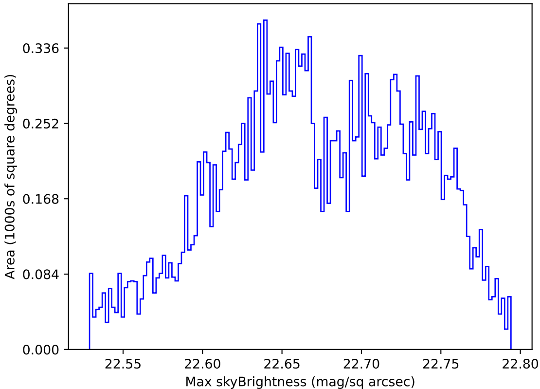
ddf_loaded_fl2_v3.4_10yrs Yr 1 u band: Max skyBrightness
