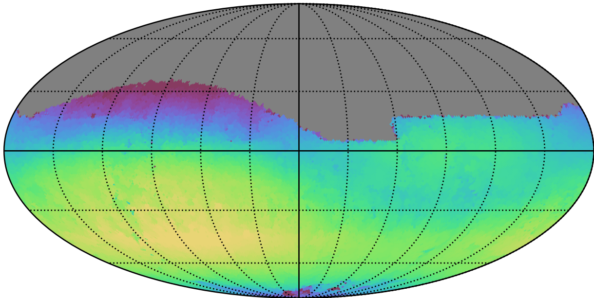
ddf_loaded_fl2_v3.4_10yrs Yr1 r band: Max skyBrightness
