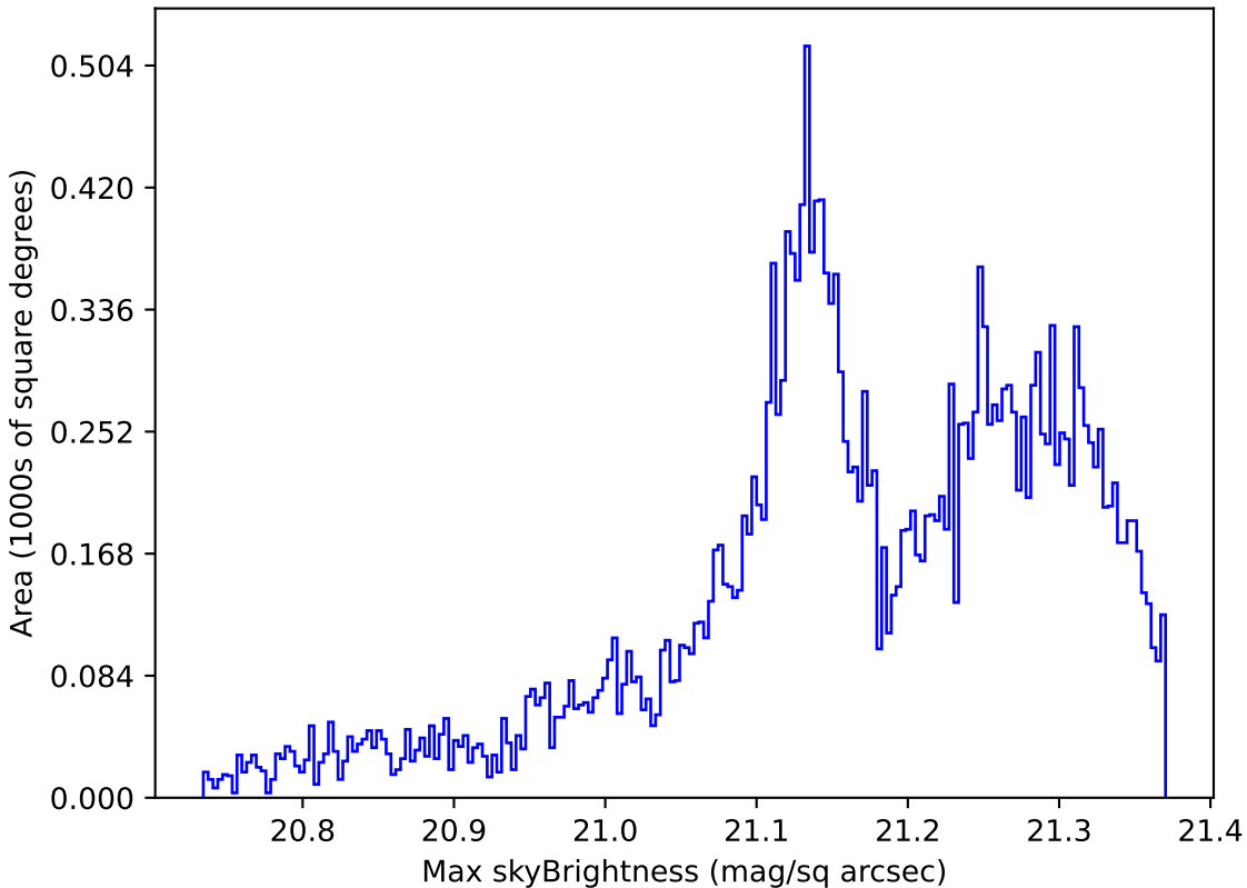
ddf_loaded_fl2_v3.4_10yrs Yr 1 r band: Max skyBrightness
