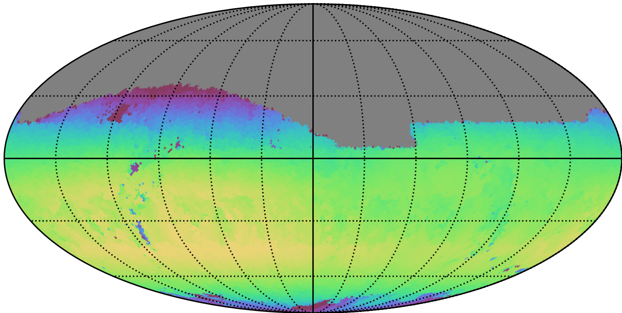
ddf_loaded_fl2_v3.4_10yrs Yr 1 i band: Max skyBrightness
