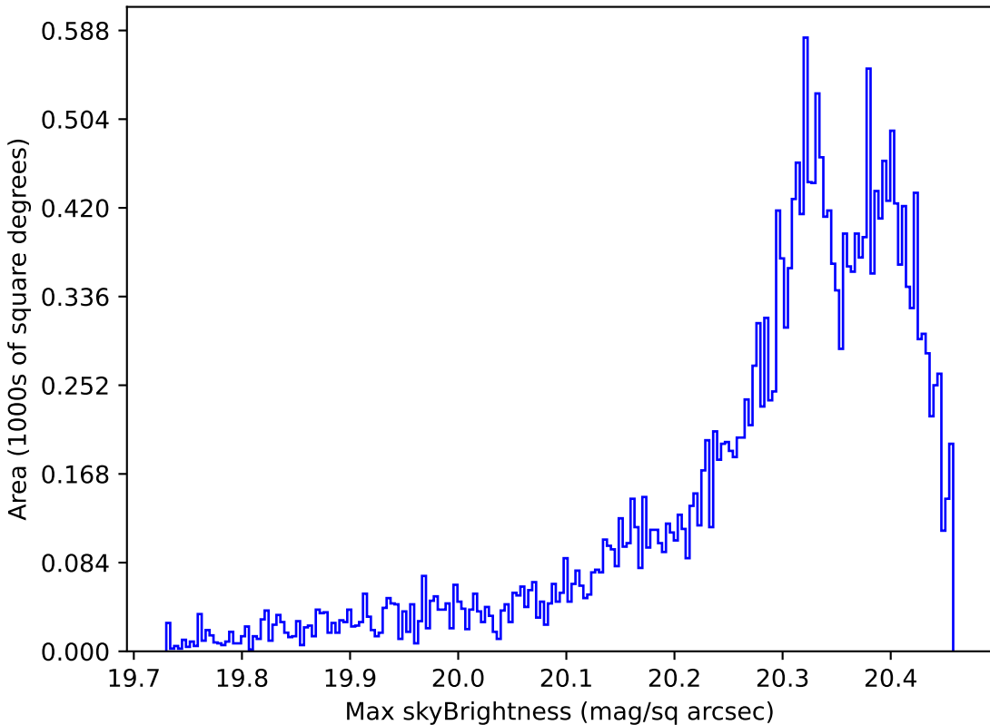
ddf_loaded_fl2_v3.4_10yrs Yr 1 i band: Max skyBrightness
