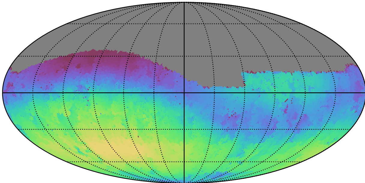
ddf_loaded_fl2_v3.4_10yrs Yr 1 g band: Max skyBrightness
