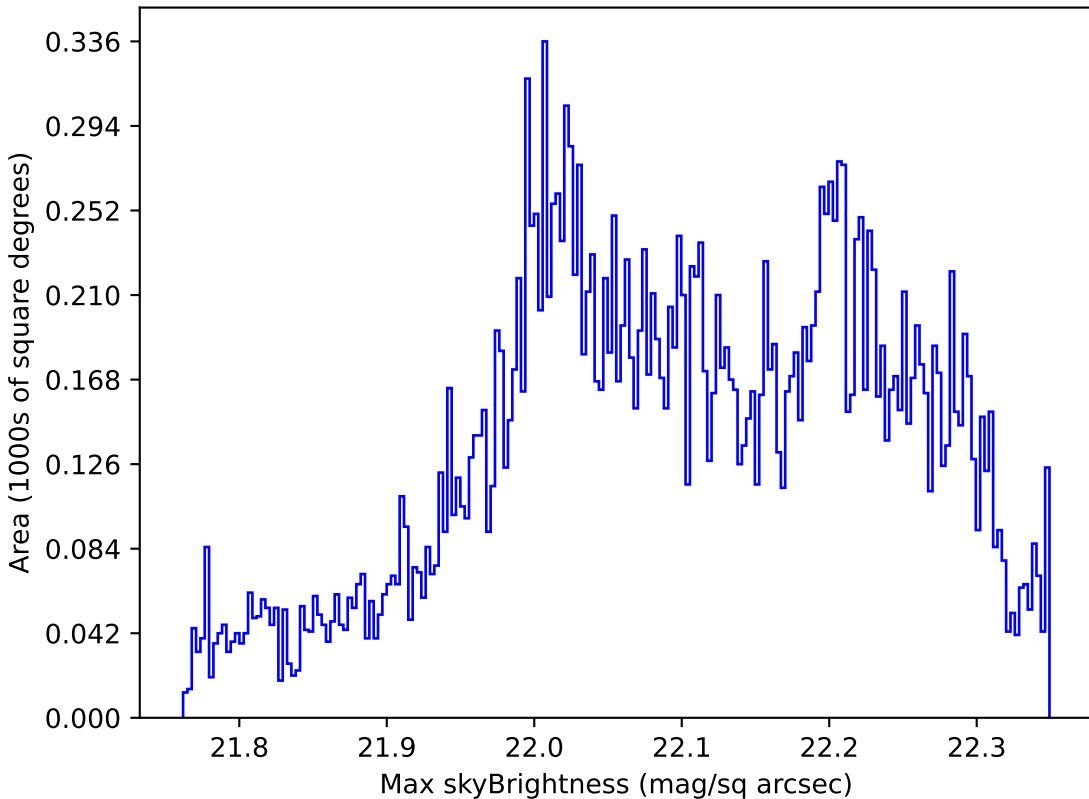
ddf_loaded_fl2_v3.4_10yrs Yr 1 g band: Max skyBrightness
