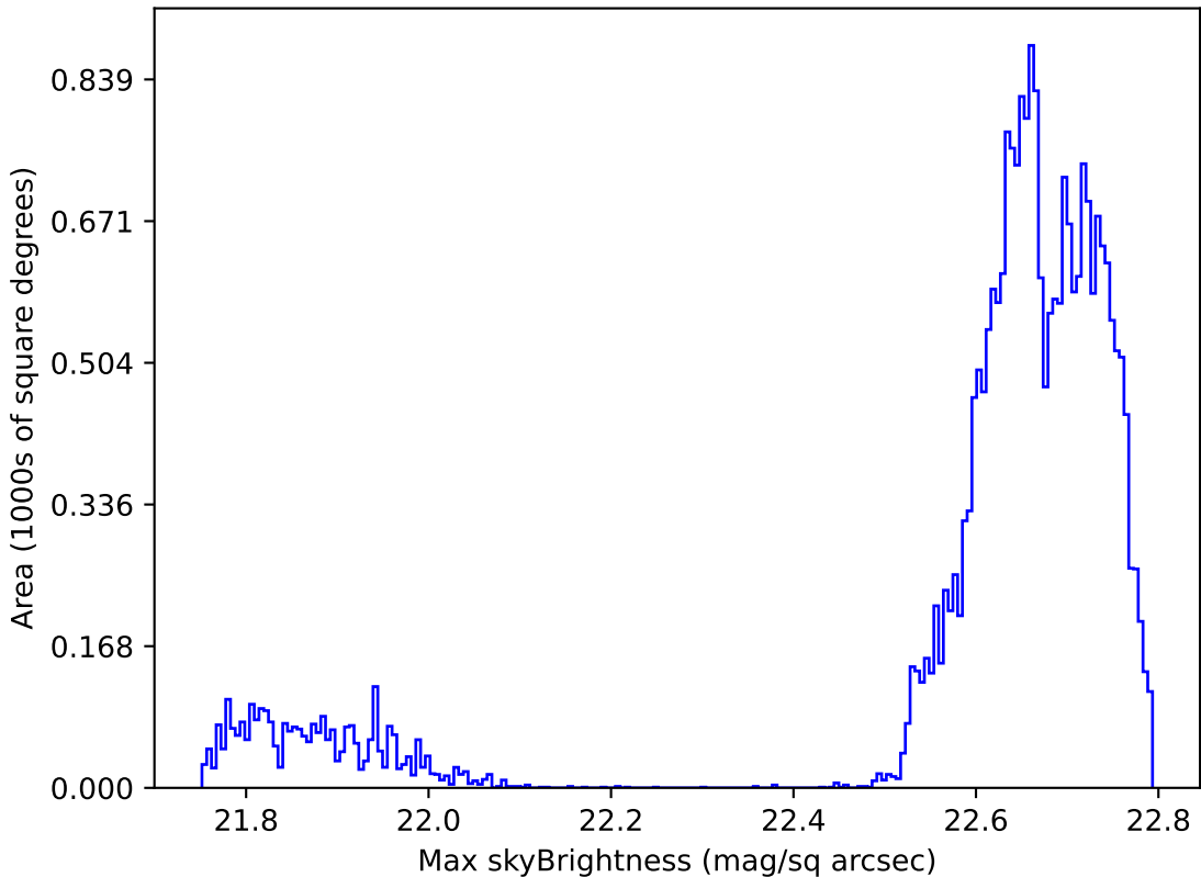
ddf_loaded_fl2_v3.4_10yrs Yr 1 all bands: Max skyBrightness
