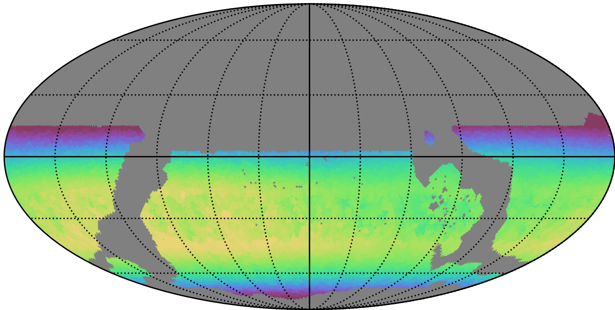
ddf_loaded_fl2_v3.4_10yrs WFD z band: Max skyBrightness
