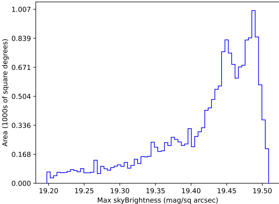
ddf_loaded_fl2_v3.4_10yrs WFD z band: Max skyBrightness
