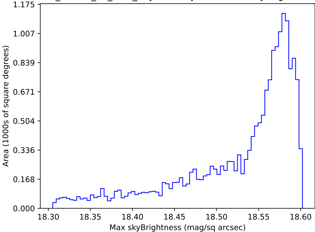
ddf_loaded_fl2_v3.4_10yrs WFD y band: Max skyBrightness
