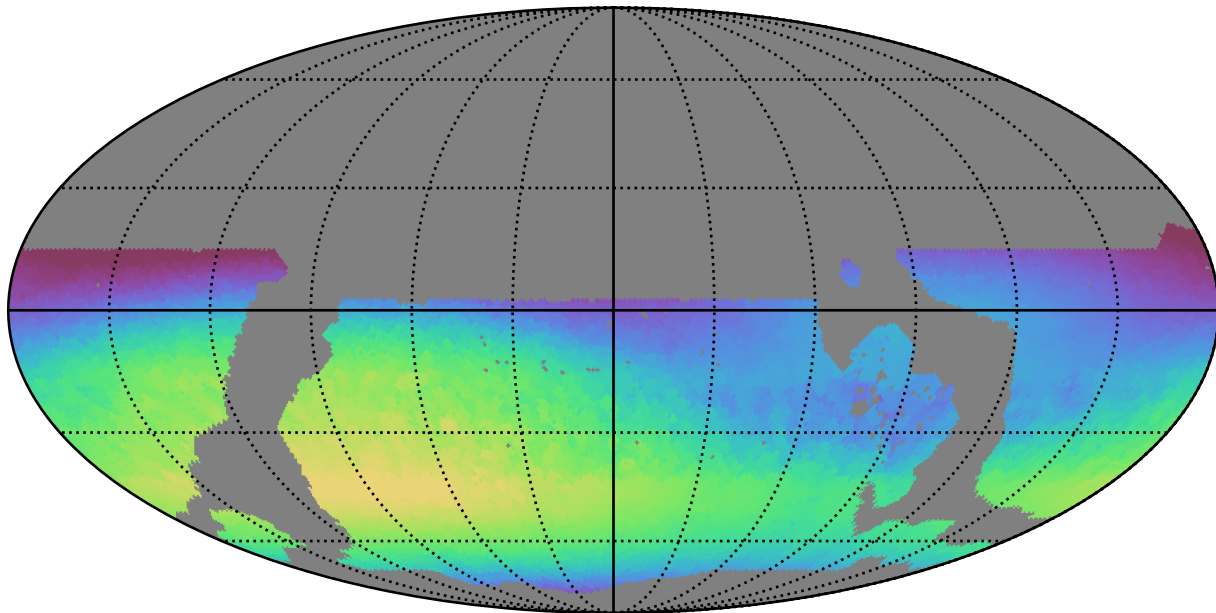
ddf_loaded_fl2_v3.4_10yrs WFD u band: Max skyBrightness
