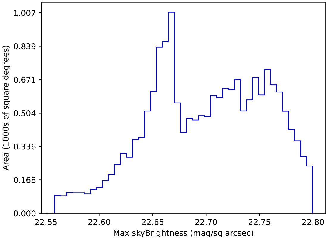
ddf_loaded_fl2_v3.4_10yrs WFD u band: Max skyBrightness
