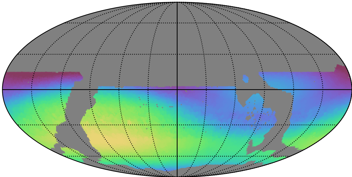
ddf_loaded_fl2_v3.4_10yrs WFD r band: Max skyBrightness
