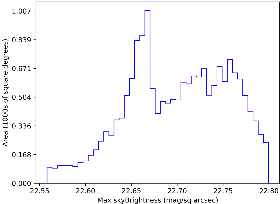
ddf_loaded_fl2_v3.4_10yrs WFD all bands: Max skyBrightness
