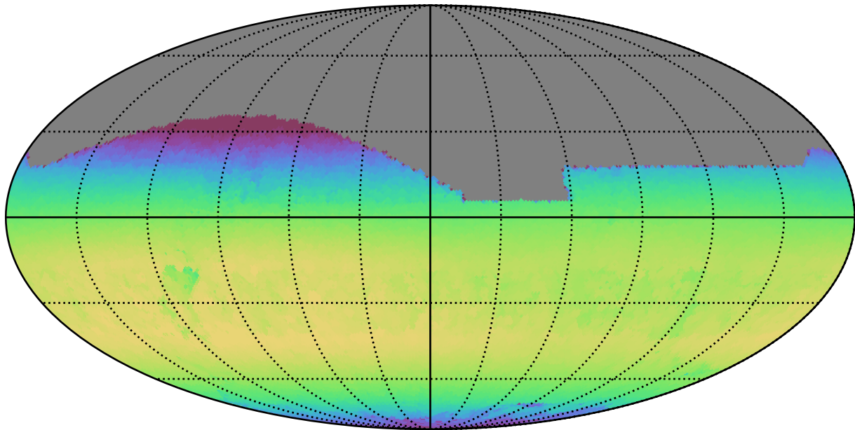
ddf_loaded_fl2_v3.4_10yrs All sky z band: Max skyBrightness
