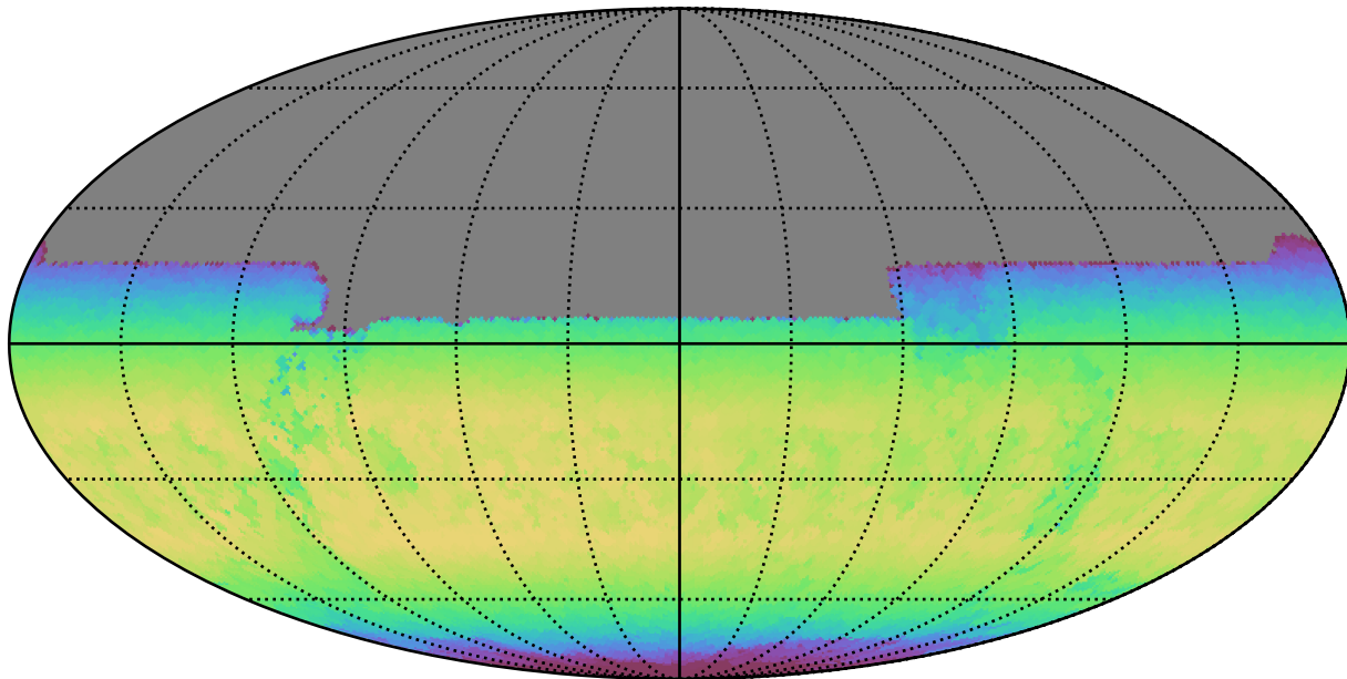
ddf_loaded_fl2_v3.4_10yrs All sky y band: Max skyBrightness
