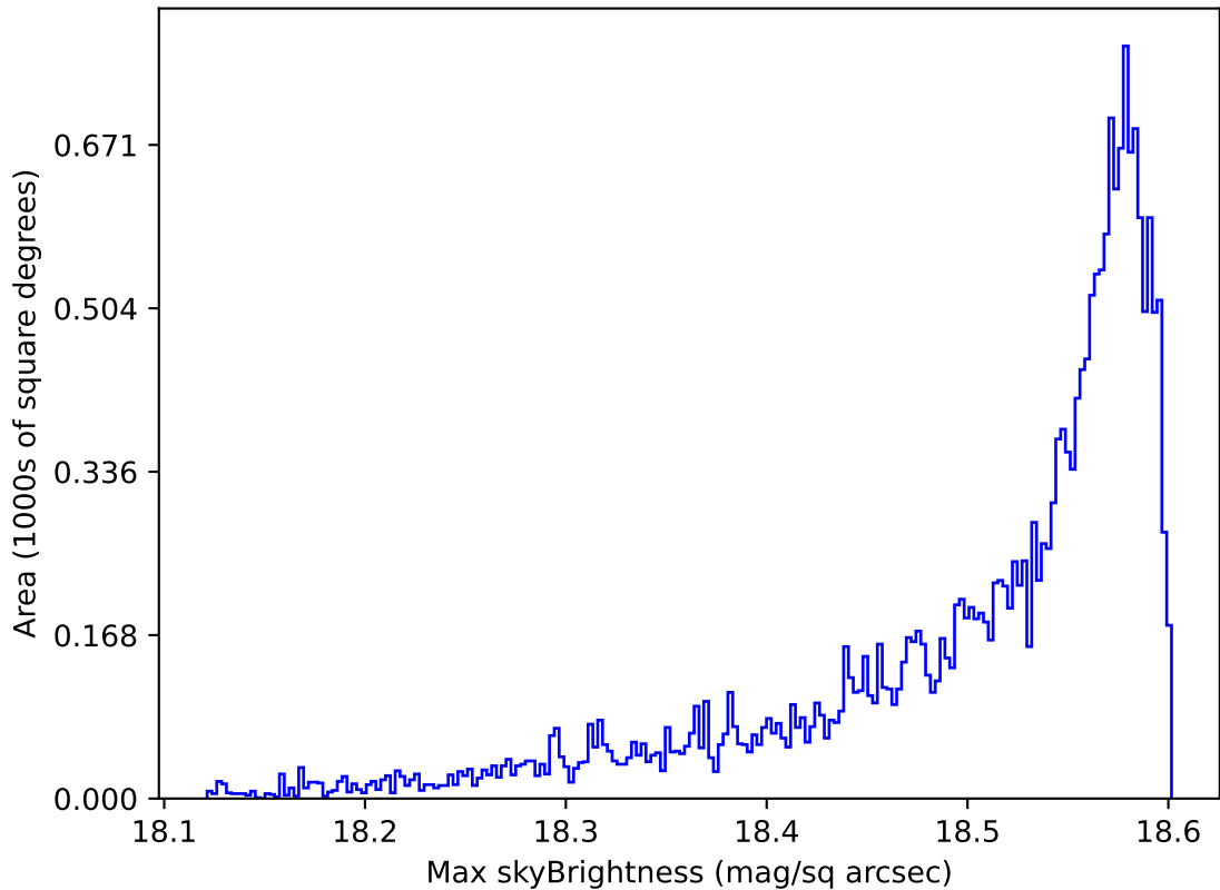
ddf_loaded_fl2_v3.4_10yrs All sky y band: Max skyBrightness
