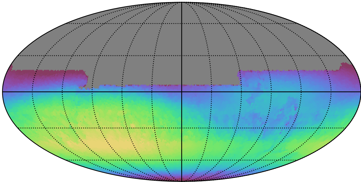
ddf_loaded_fl2_v3.4_10yrs All sky u band: Max skyBrightness
