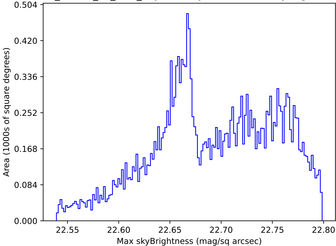
ddf_loaded_fl2_v3.4_10yrs All sky u band: Max skyBrightness
