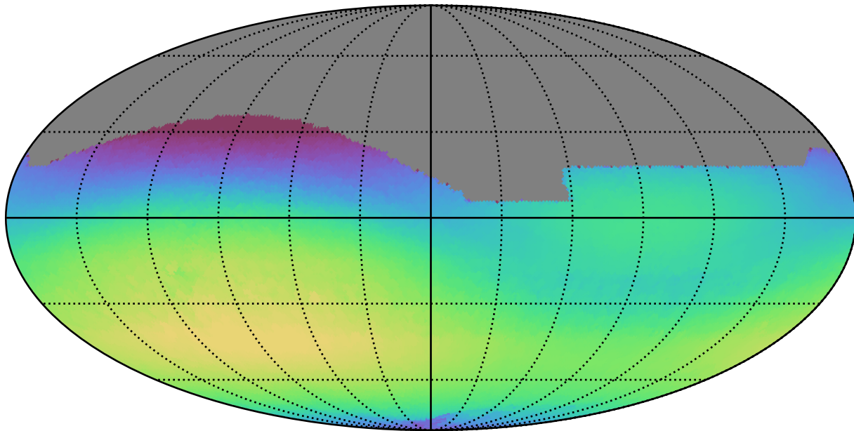
ddf_loaded_fl2_v3.4_10yrs All sky r band: Max skyBrightness
