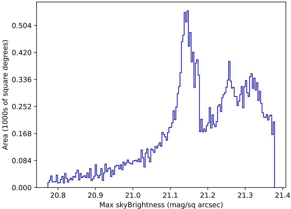
ddf_loaded_fl2_v3.4_10yrs All sky r band: Max skyBrightness
