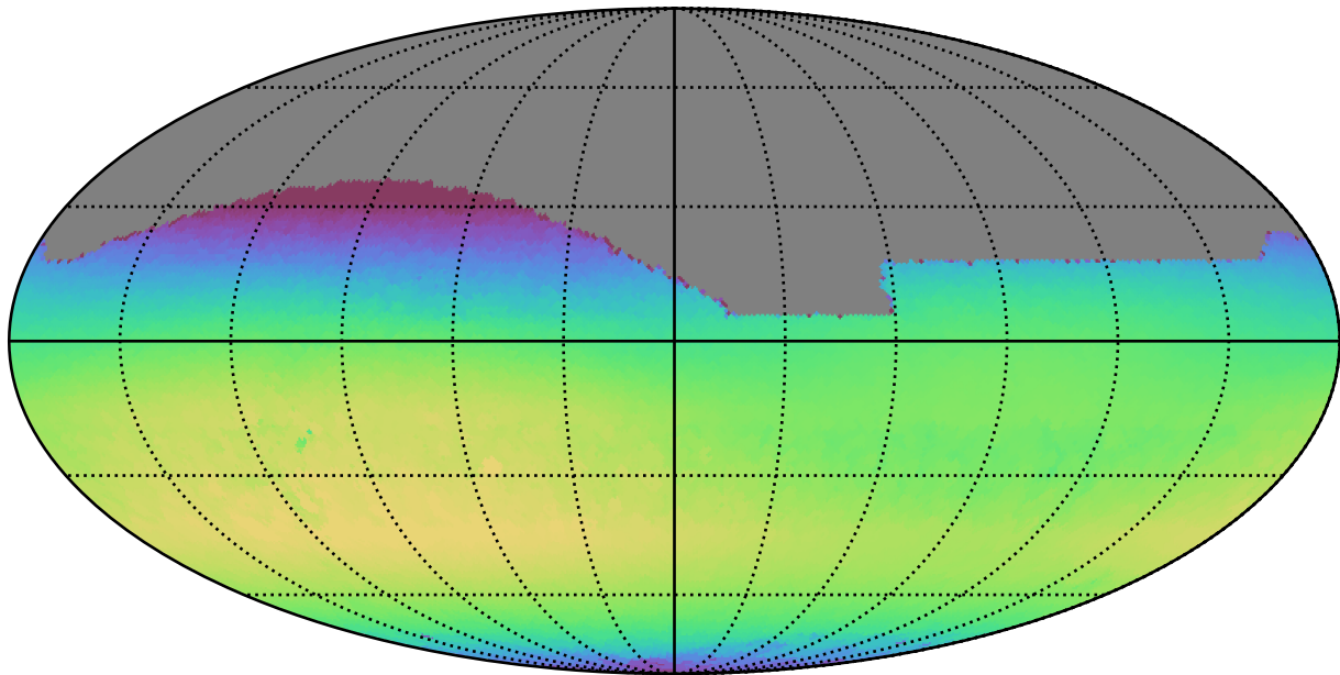
ddf_loaded_fl2_v3.4_10yrs All sky i band: Max skyBrightness
