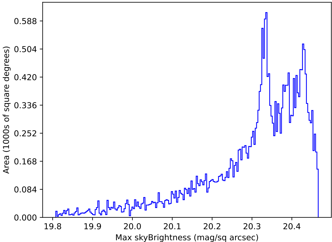
ddf_loaded_fl2_v3.4_10yrs All sky i band: Max skyBrightness
