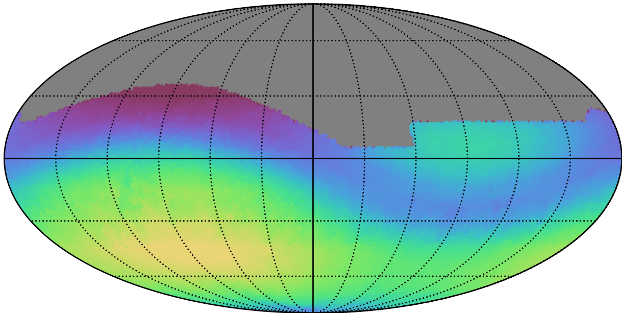
ddf_loaded_fl2_v3.4_10yrs All sky g band: Max skyBrightness
