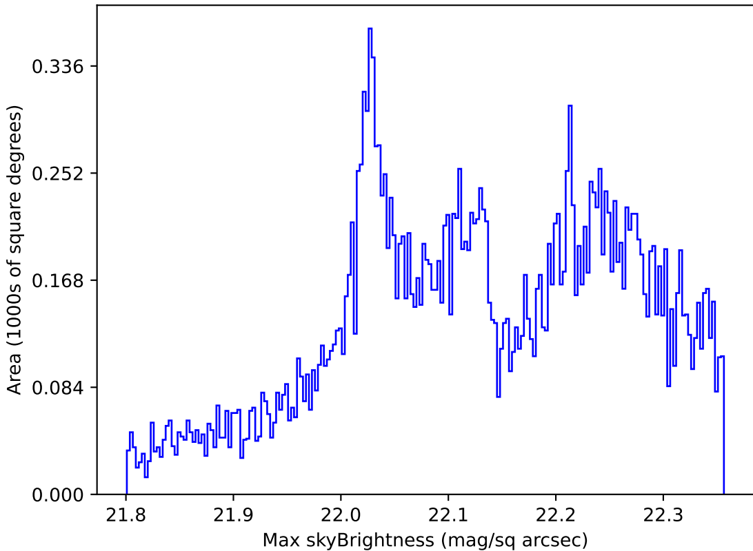
ddf_loaded_fl2_v3.4_10yrs All sky g band: Max skyBrightness
