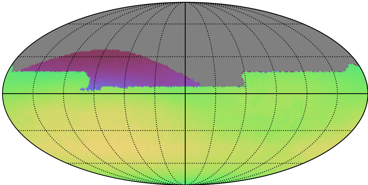
ddf_loaded_fl2_v3.4_10yrs All sky all bands: Max skyBrightness
