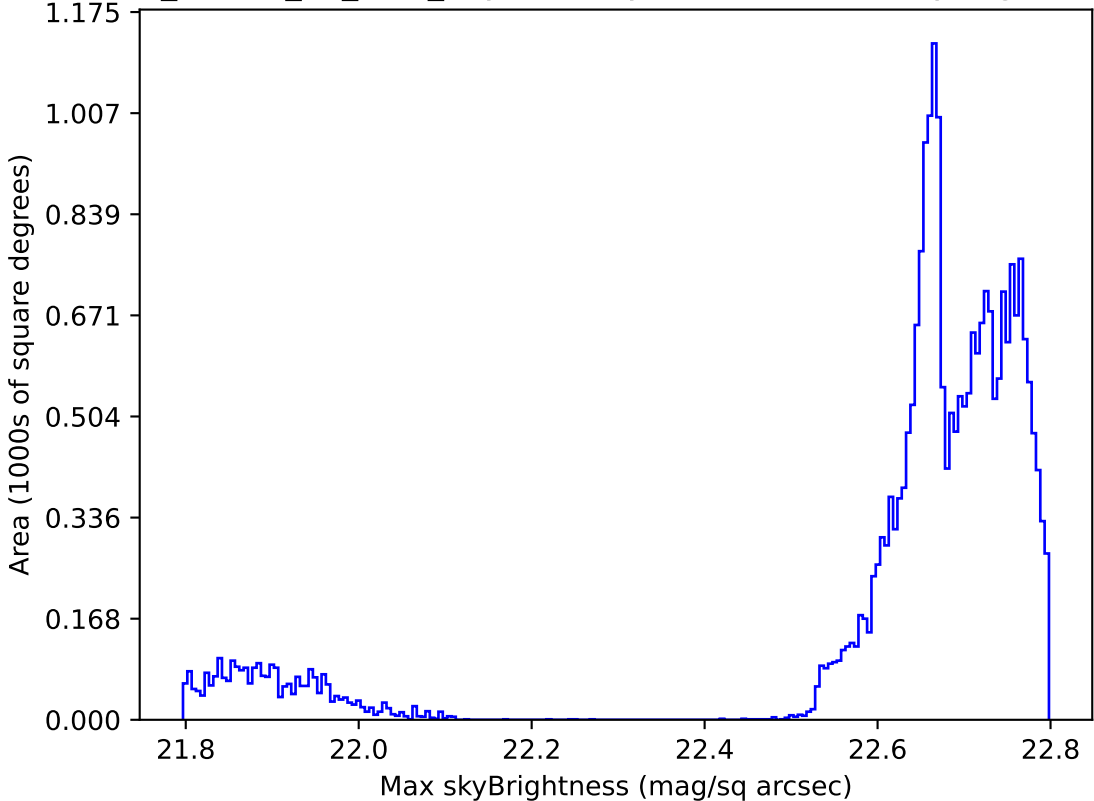
ddf_loaded_fl2_v3.4_10yrs All sky all bands: Max skyBrightness
