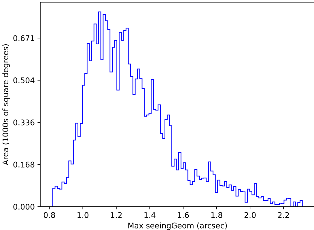
ddf_loaded_fl2_v3.4_10yrs Yr 1 z band: Max seeingGeom
