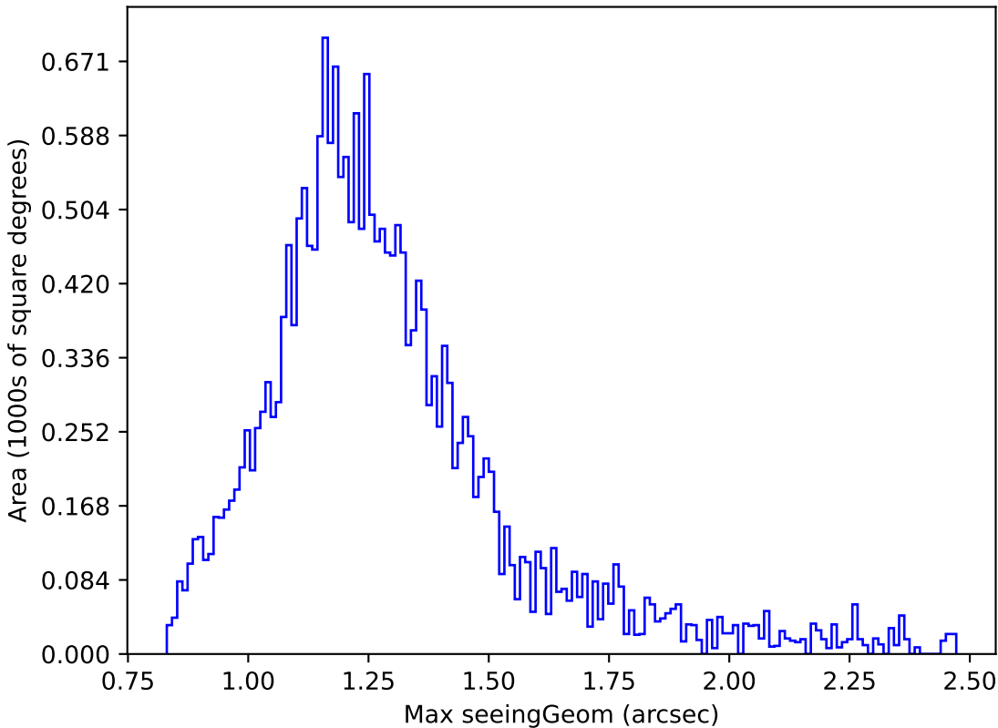
ddf_loaded_fl2_v3.4_10yrs Yr 1 y band: Max seeingGeom
