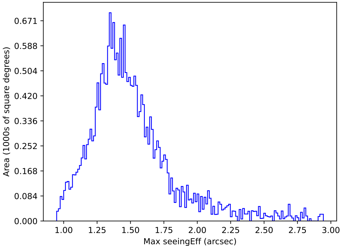
ddf_loaded_fl2_v3.4_10yrs Yr 1 y band: Max seeingEff
