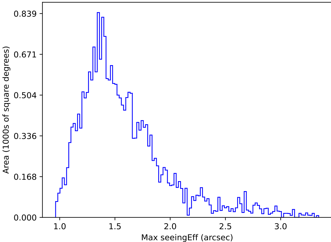
ddf_loaded_fl2_v3.4_10yrs Yr 1 u band: Max seeingEff
