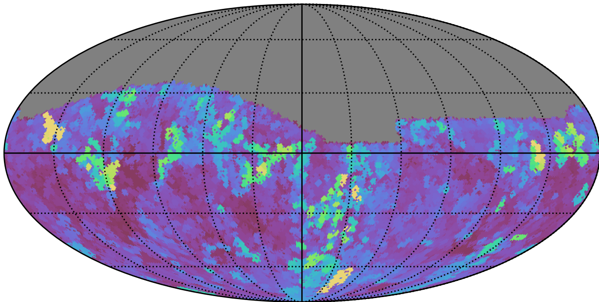
ddf_loaded_fl2_v3.4_10yrs Yr 1 i band: Max seeingEff
