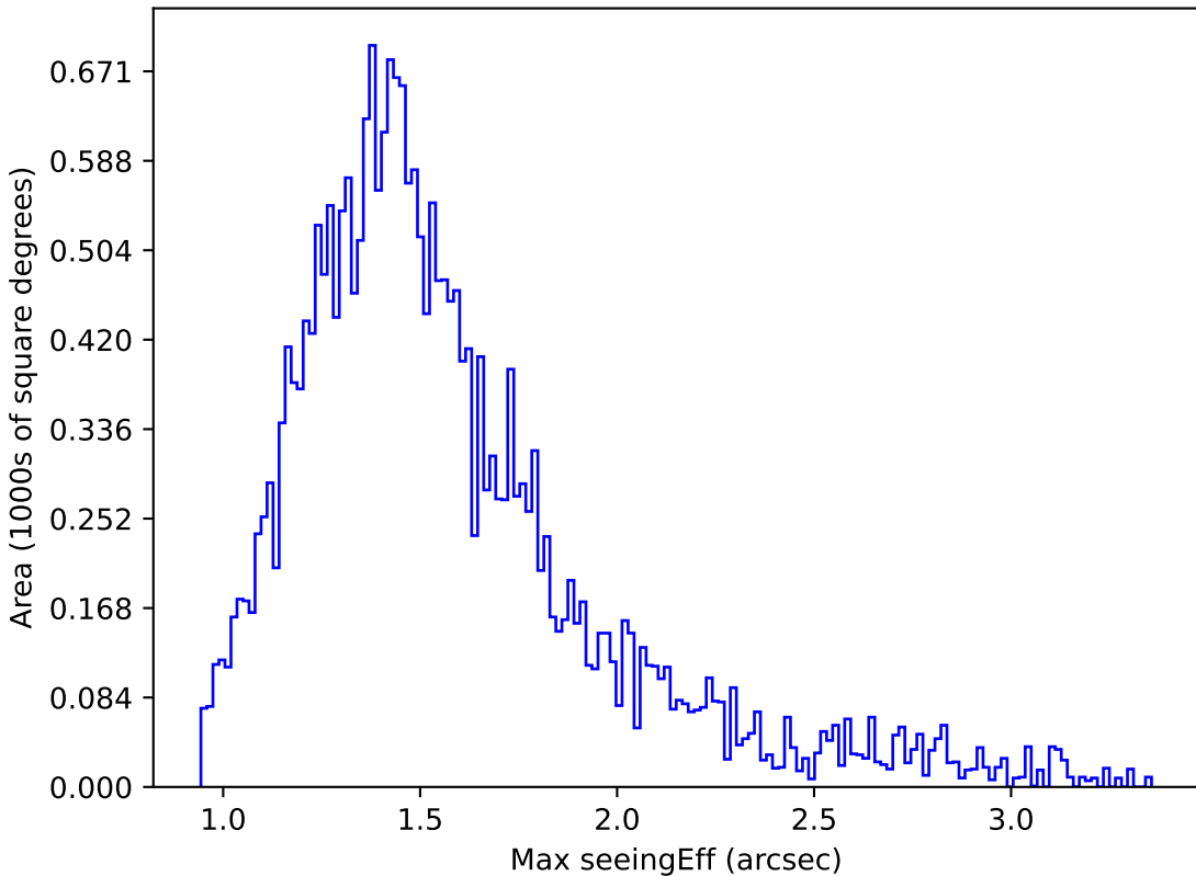
ddf_loaded_fl2_v3.4_10yrs Yr 1 i band: Max seeingEff
